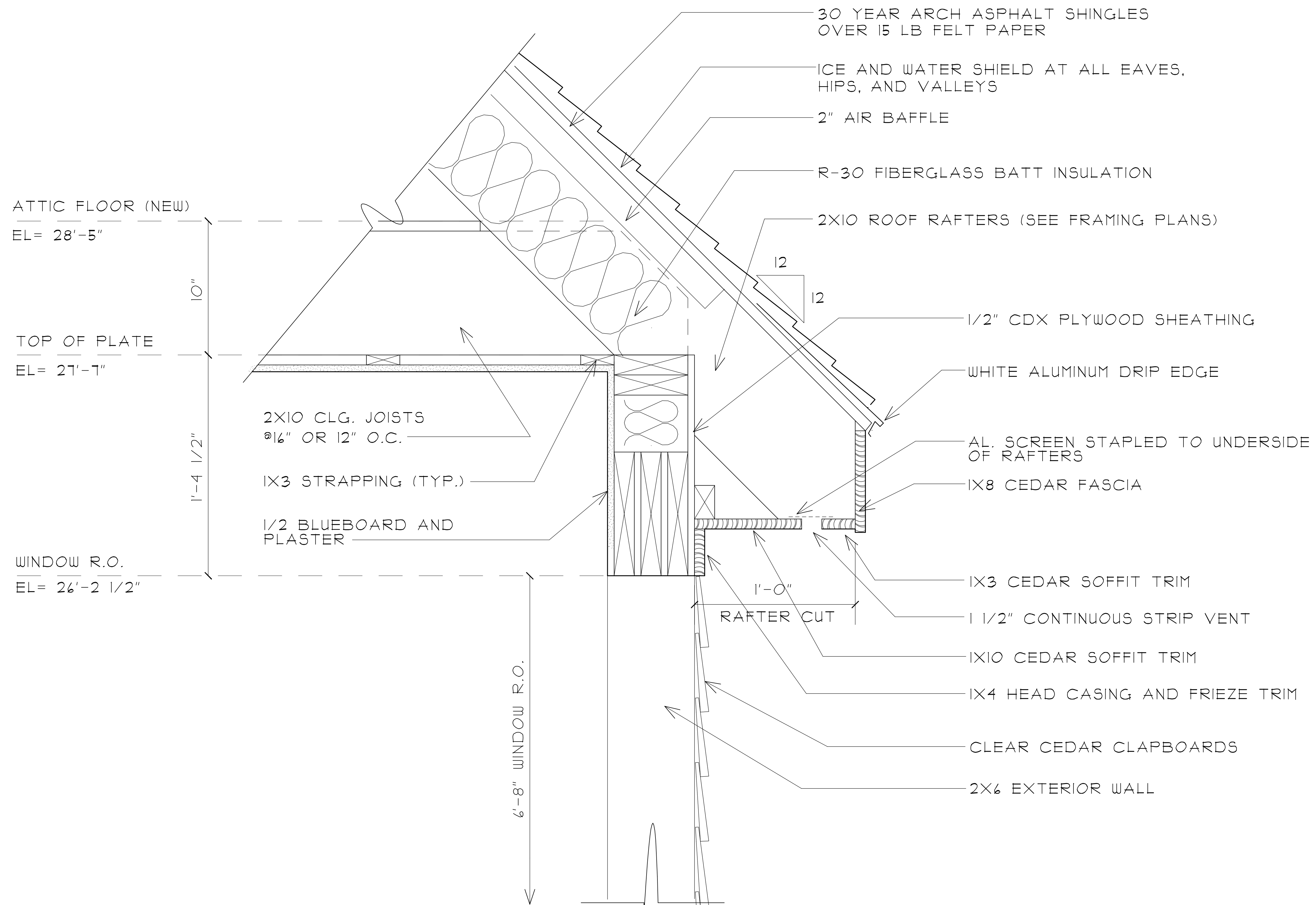
2 EAVE DETAIL-MAIN HOUSE SCALE: 1 1/2" = 1'-0"
